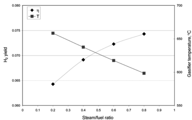
Fig. 4. H_2 yield and gasifier temperature versus the steam/fuel ratio.
